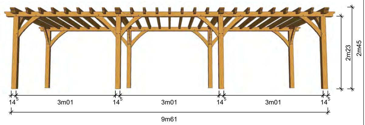
Oak structure Post 145x145
