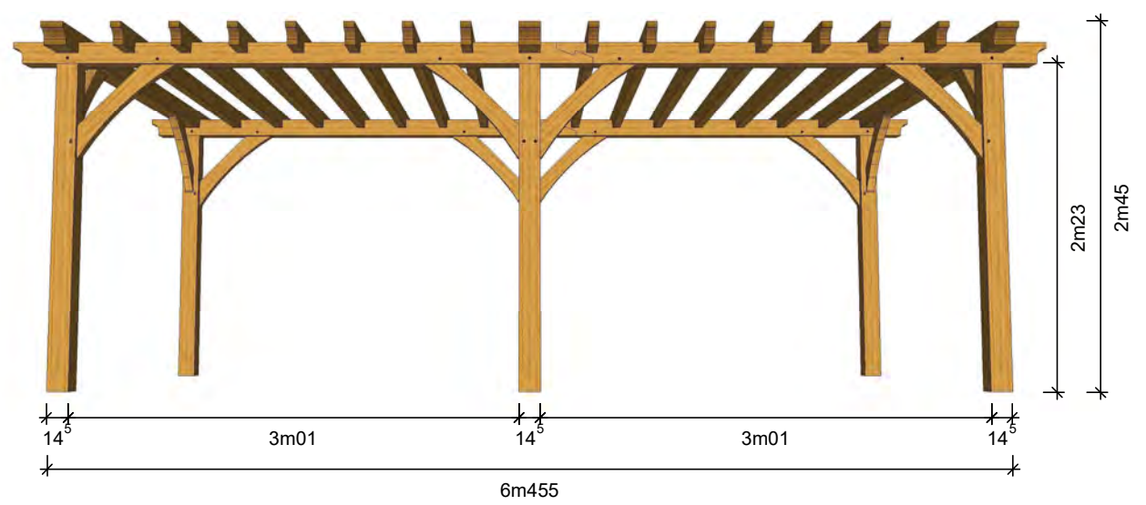
Oak structure Post 145x145
