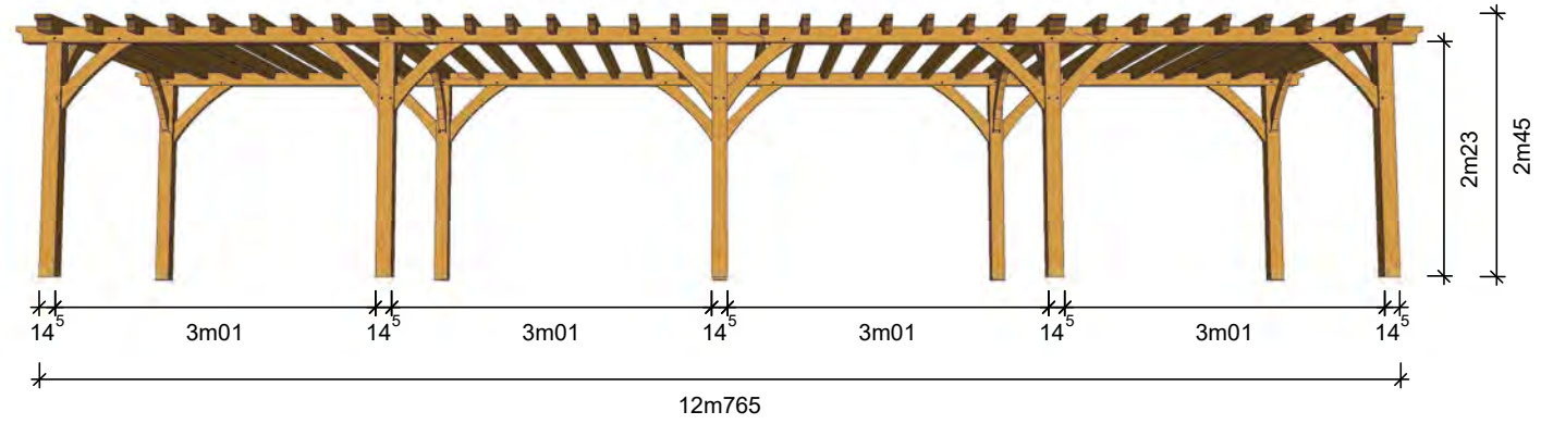
Oak structure Post 145x145
